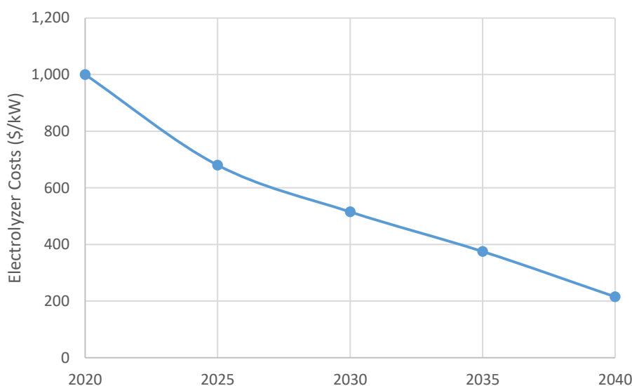
Figure 30. Installed Capacity Cost of Electrolyzers, $/kW, 2020-2040
