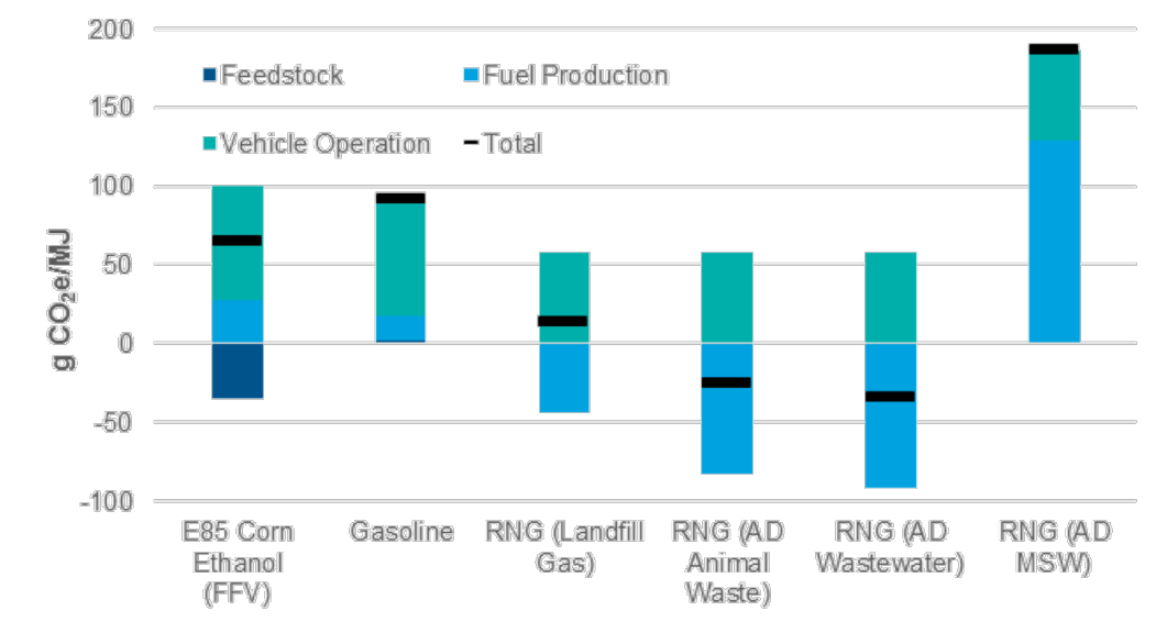
Figure 35. Summary of carbon intensities for transportation fuels across life-cycle stages (ANL 2019).
