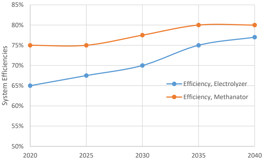
Figure 25. Assumed Efficiency for Electrolysis and Methanation, 2020-2040
